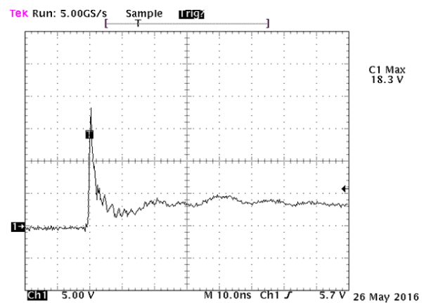
TLP Curve
